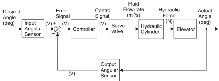
Fig. 1.9 Block diagram of elevator control system.
