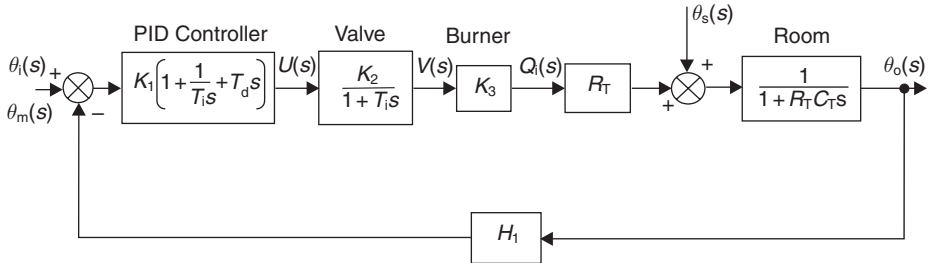
Fig. 4.33 Block diagram of temperature control system.
